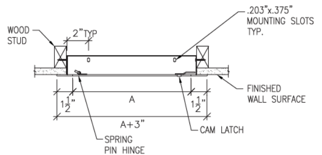
Section Detail
