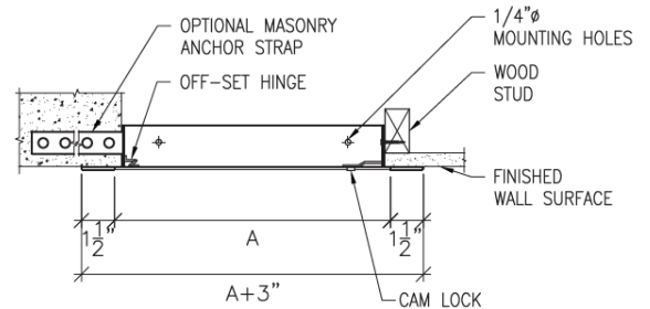
Section Detail
