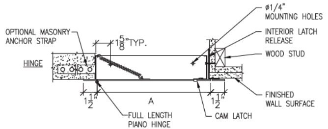
Section Detail
