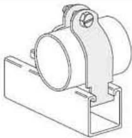
Fig. 2001-2016 IRON PIPE CLAMP
