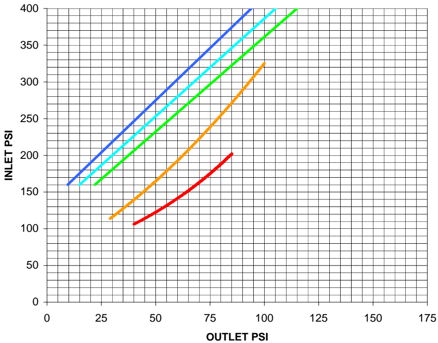
URFA-20S-2.5 (500 GPM)
