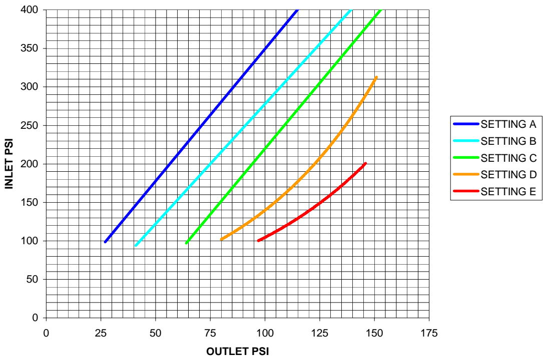
URFA-20S-2.5 (50 GPM)
