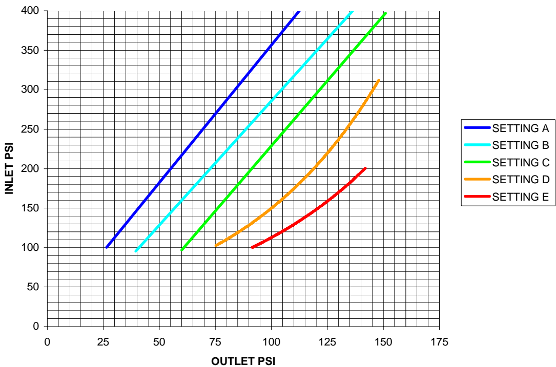
URFA-20S-2.5 (100 GPM)
