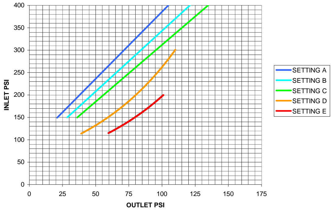
URFA-20S-2.5 (400 GPM)
