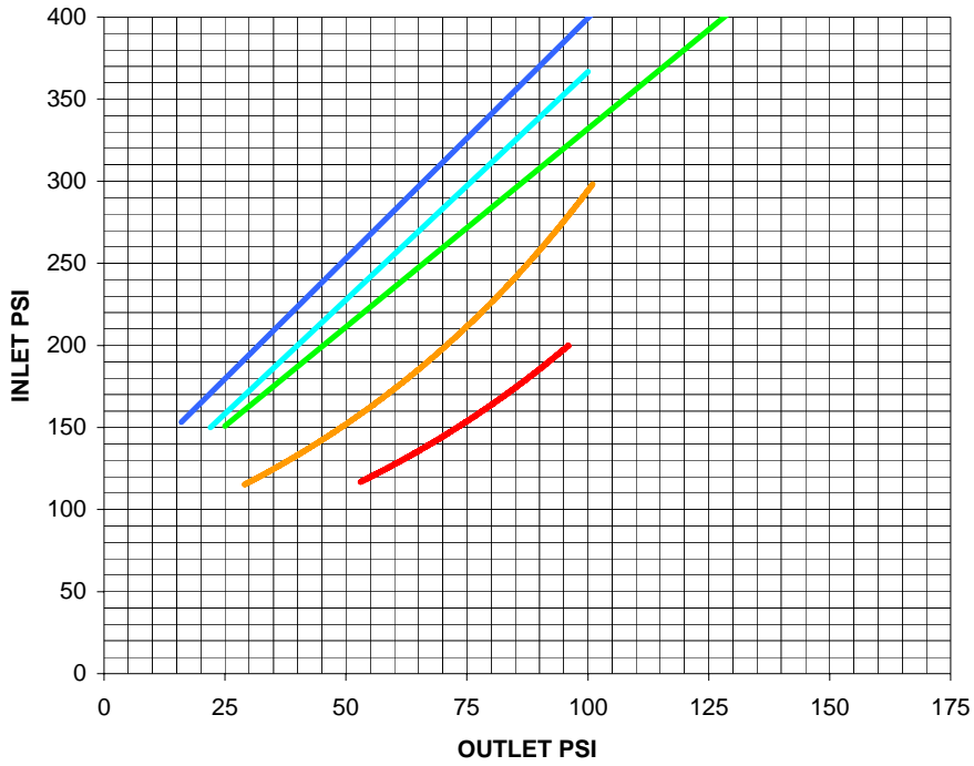
URFA-20S-2.5 (450 GPM)
