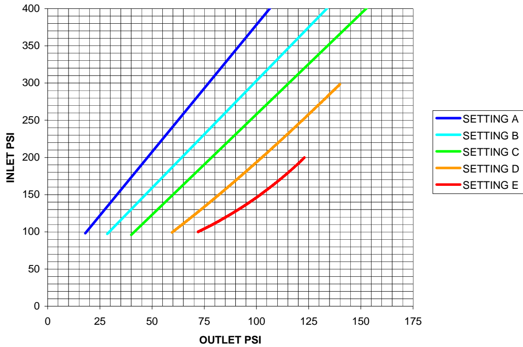
URFA-20-2.5 URFA-25-2.5 (250 GPM)
