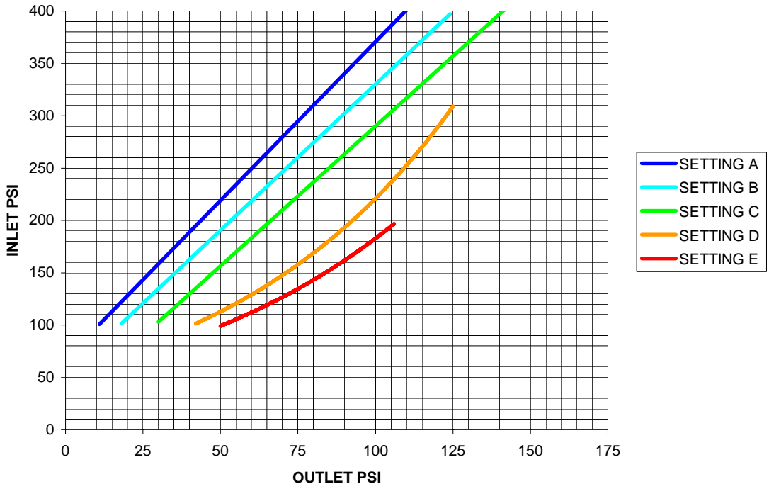
URFA-20S-2.5 (350 GPM)
