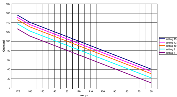
A155-A156 1-1/2" 70 gpm 100 ft hose
