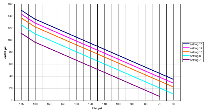
A155-A156 1-1/2" 80 gpm 100 ft hose
