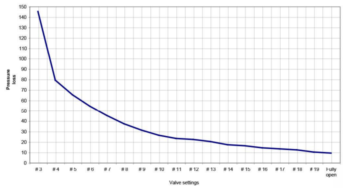
A155 A156 2-1/2" size. Pressure loss at 250 gpm
