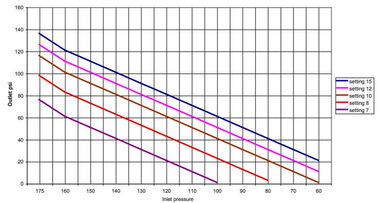
A155-A156 1-1/2" 100 gpm 100 ft hose
