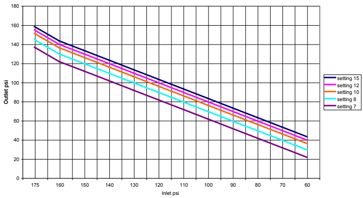
A155-A156 1-1/2" 60 gpm 100 ft hose
