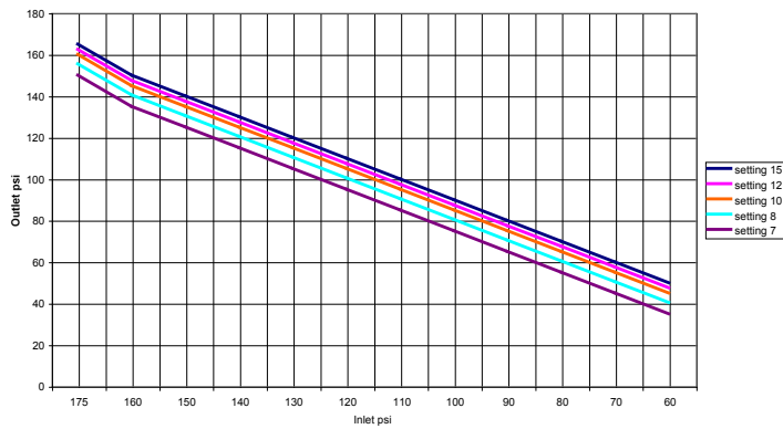
A155-A156 1-1/2" 50 gpm 100 ft hose
