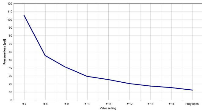
Pressure loss 1-1/2" A155- A156 while flowing 100 gpm
