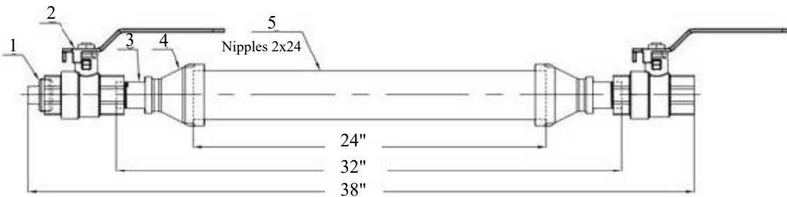
Figure 2 Drum Drip 2x1x24 Product Structure PT#: DDE224R
