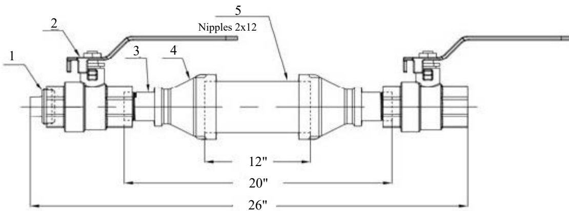
Figure 1 Drum Drip 2x1x12 Product Structure PT#: DDE212R
