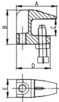
PT#: 3640G-NFE 3/8" Galvanized Small Mouth
