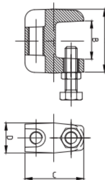
PT#: 3641-NFE 3/8" Wide Mouth
