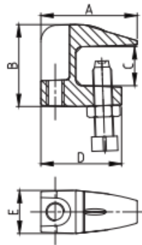
PT#: 3640-NFE 3/8" Small Mouth
