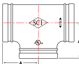
Fig. 65TS & 66TS Tee, Short Radius
