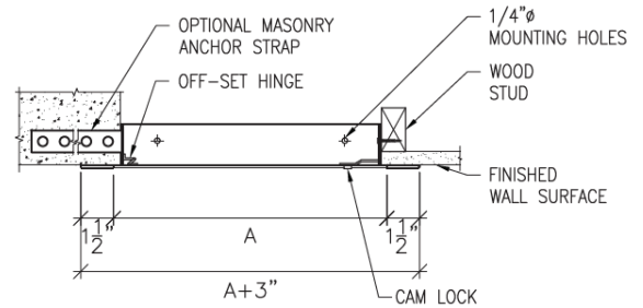
Section Detail
