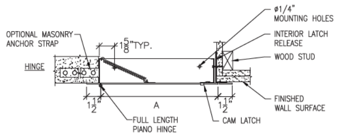
Section Detail
