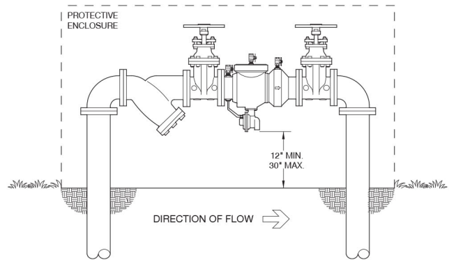
OUTDOOR INSTALLATION
