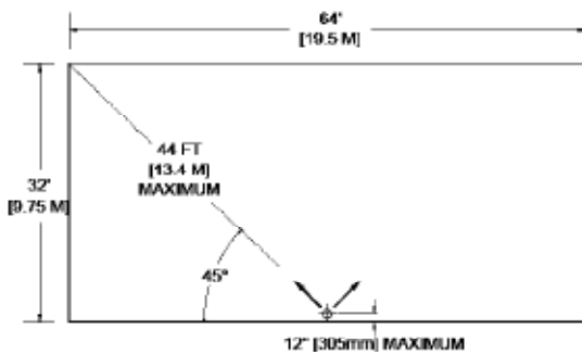
180° Sidewall Nozzle (2 Port) Arrangement
