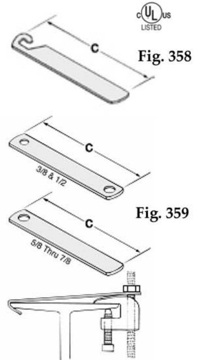
Fig. 359 RETAINING STRAP
