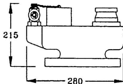
2 Way Breeching Inlet
