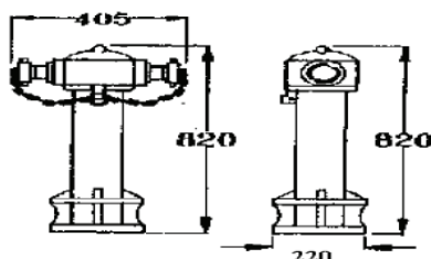
Hydrant
