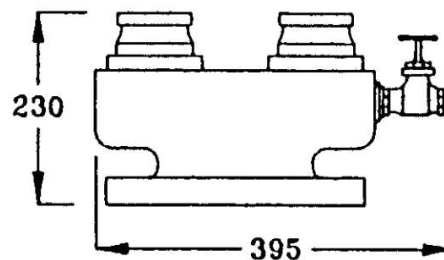
4 Way Breeching Inlet
