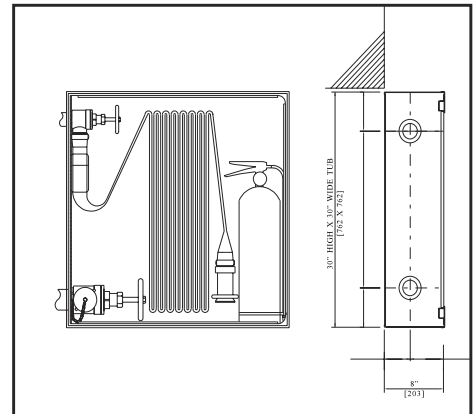
CS-800 (Double Valve with Extinguisher)
