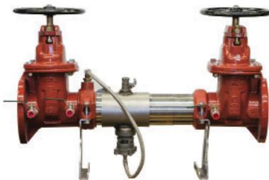
Watts 957 Reduced Pressure
