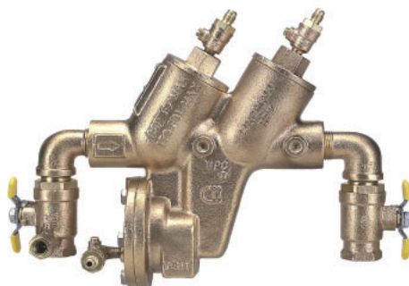
Apollo 40 - 200 Reduced Pressure
