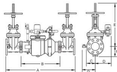
MODEL 350ADA with OS&Y option
