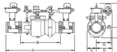
MODEL 350ADA with BGVIC option
