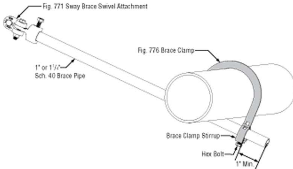
Typical Assembly (Brace Pipe Below Service Pipe)
